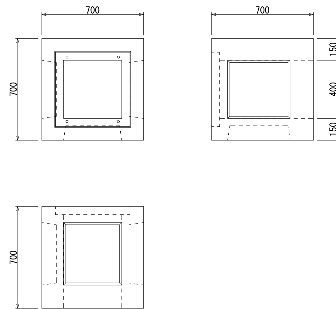
FM-400 (369kg)
