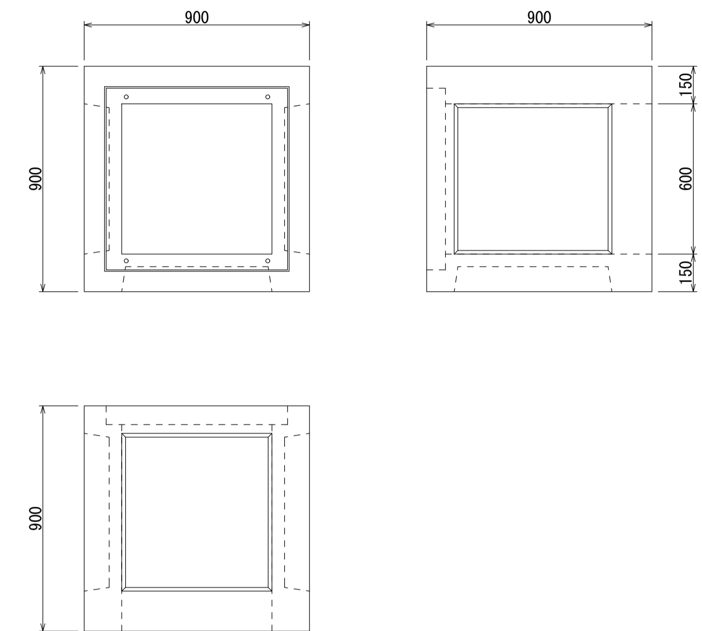
FM-600 (769kg)
